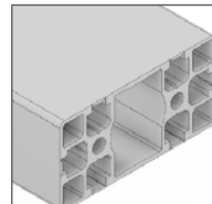
10-4590S4-0 Aluminum Profile 45MM X 90MM Smooth Sides-Tear Away
