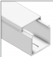
65-000-0 45MM Plastic Conduit 38MM X 38MM - Gray 6.5 FT.
